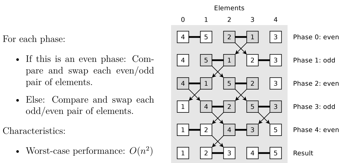
Figure 1: Odd-even sort example [1]
